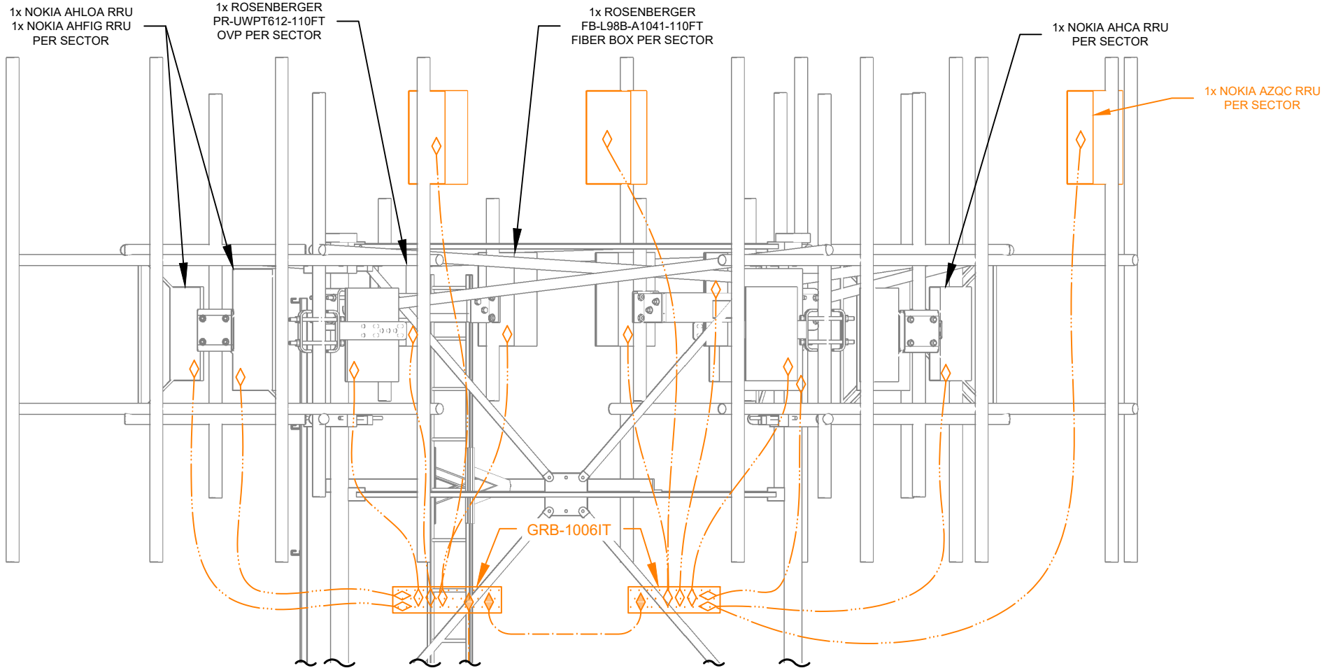
1 G1 TOWER GROUNDING ELEVATION SCALE: NO SCALE
