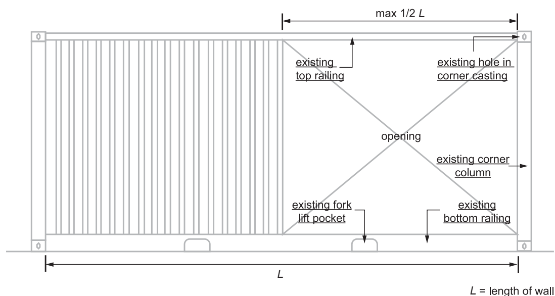
FIGURE 3114.8.5.3(1) Bracing Unit Distribution—Maximum Linear Length
