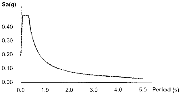
Design Horizontal Response Spectrum
