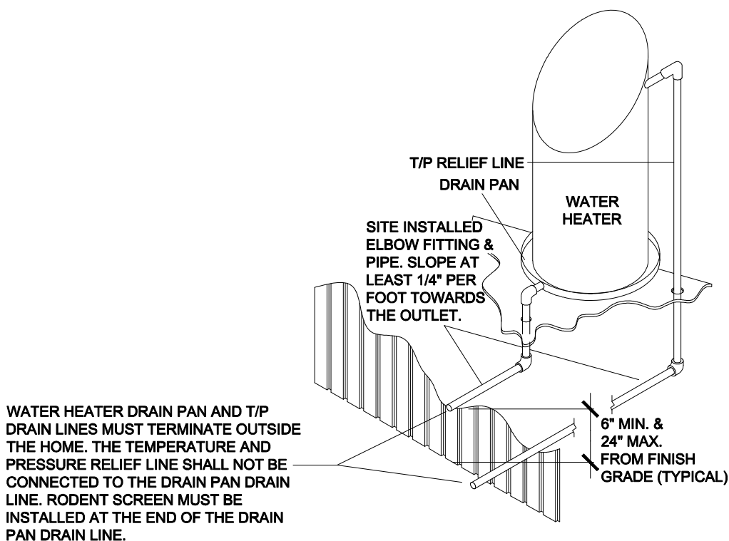
Figure 67. Water heater drip pan and drain
