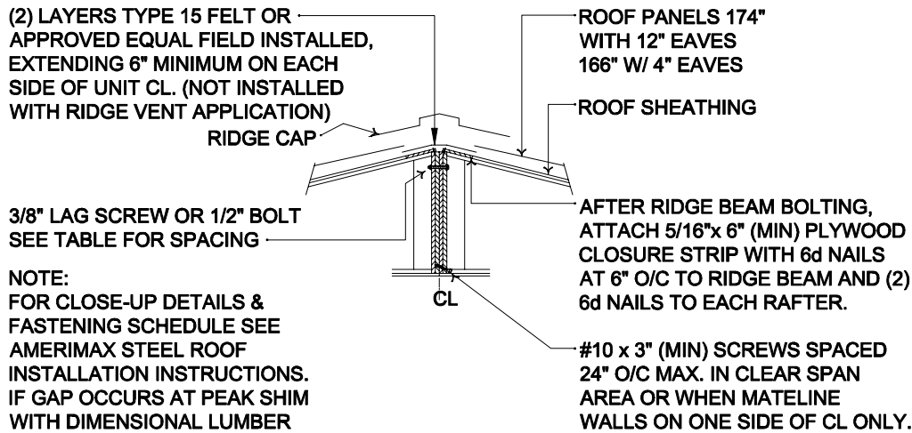
RIDGE CLOSE - UP DETAIL - METAL ROOF
