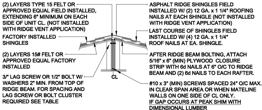
RIDGE CLOSE - UP DETAIL - SHINGLE ROOF
