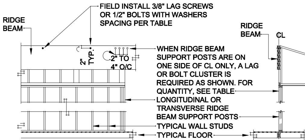
RIDGE BEAM BOLTING DETAIL
