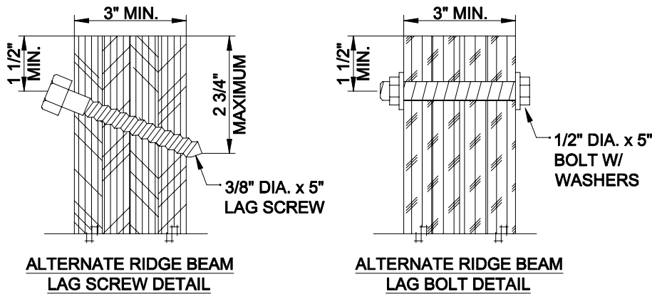
RIDGE BEAM BOLTING DETAIL
