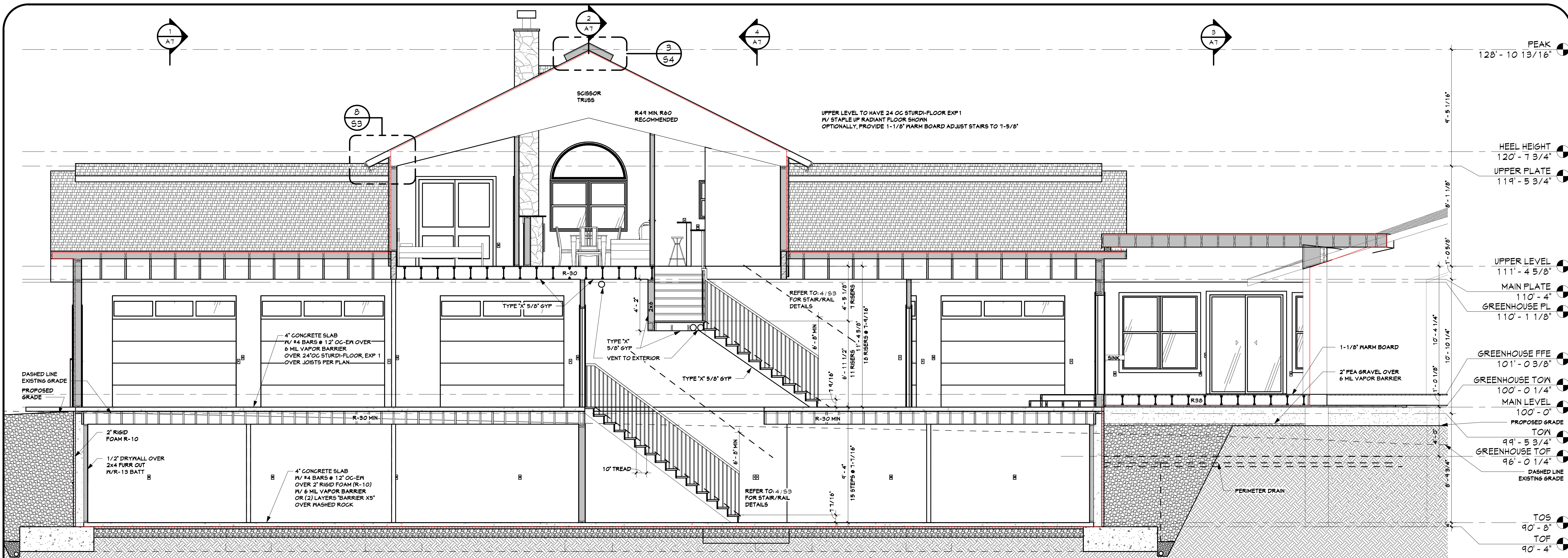
④ STAIR, ENTRY LONG SECTION 1/4" = 1'-0"
