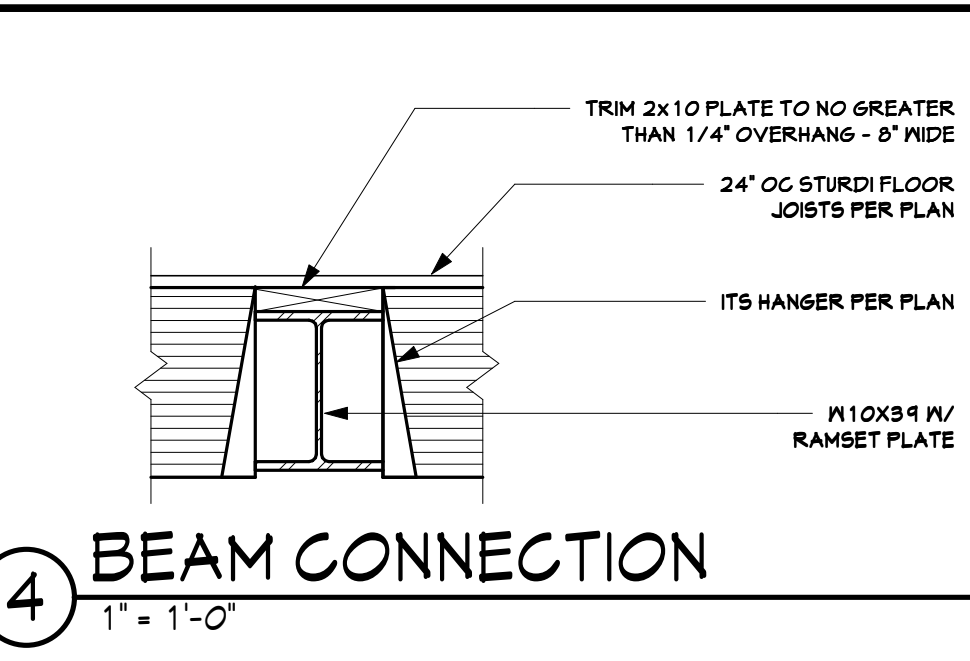
4 BEAM CONNECTION 1" = 1'-0"
