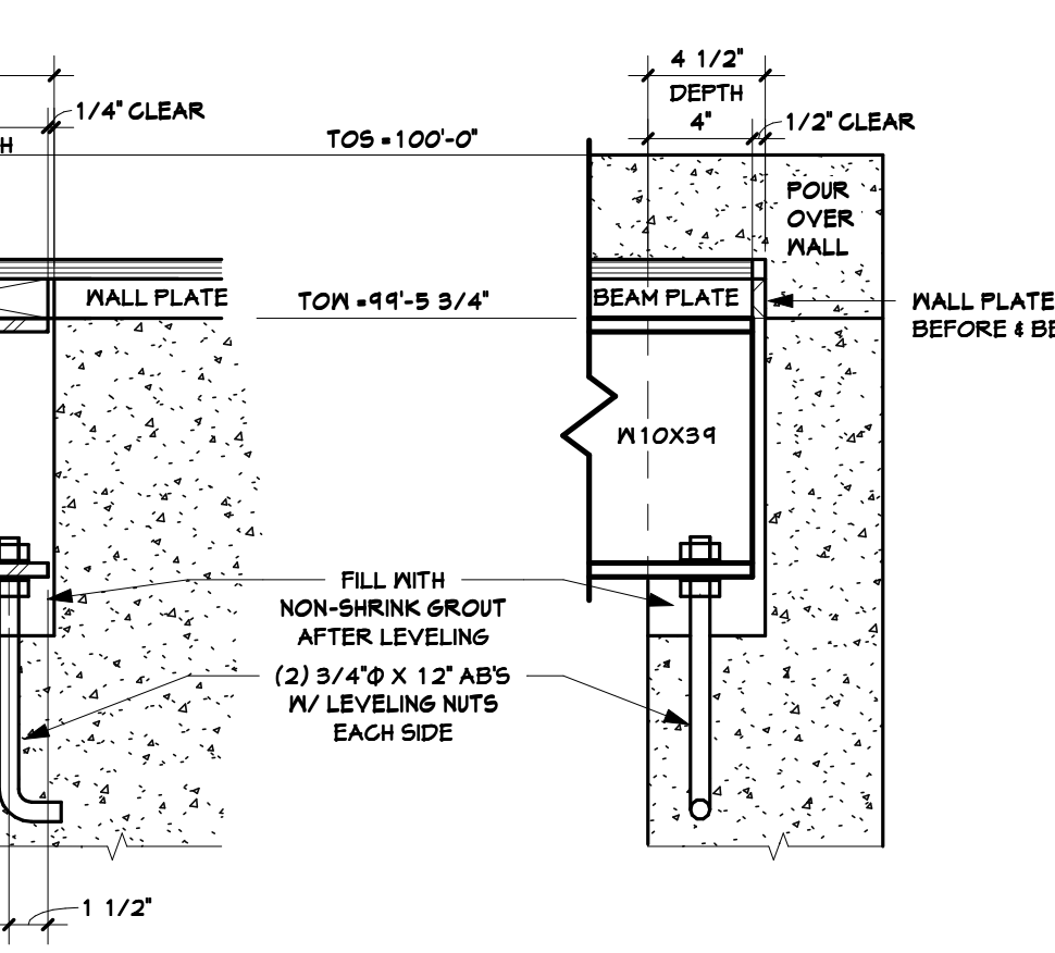
19 WALL, SLAB & FOOTER DETAIL 1/2" = 1'-0"
