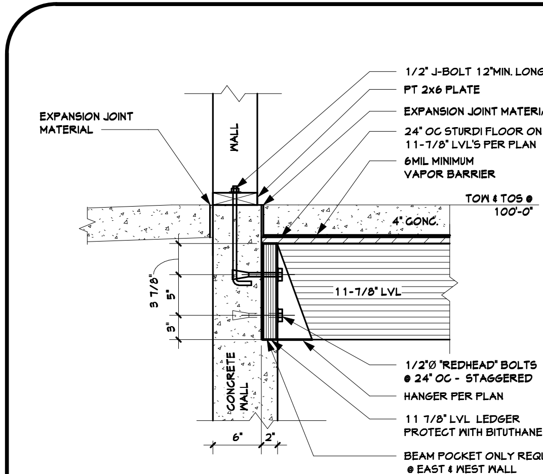
1 WEST WALL 1" = 1'-0"
