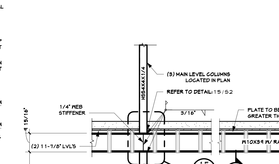
12 GRADE BEAM @ ELEVATOR PIT 1/2" = 1'-0"
