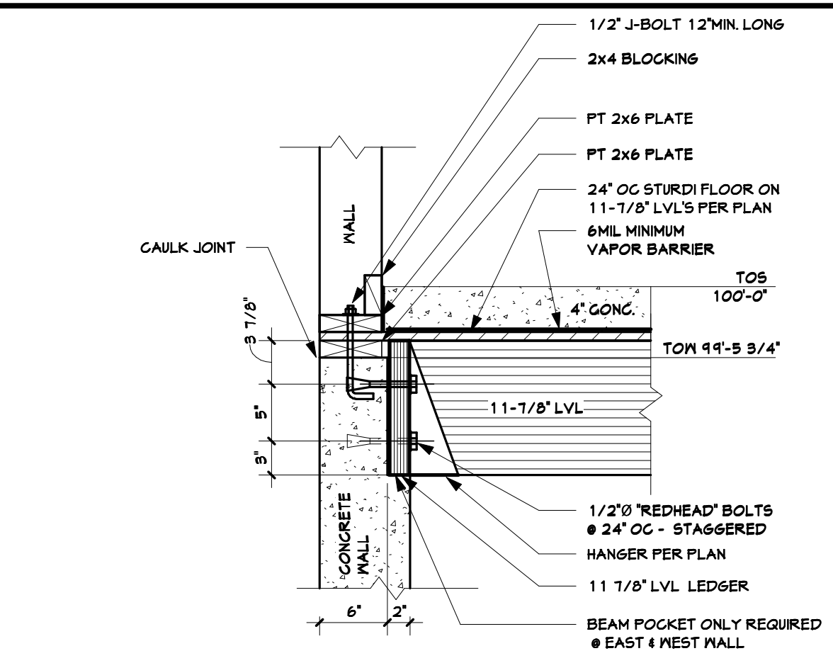
2 EAST WALL 1" = 1'-0"
