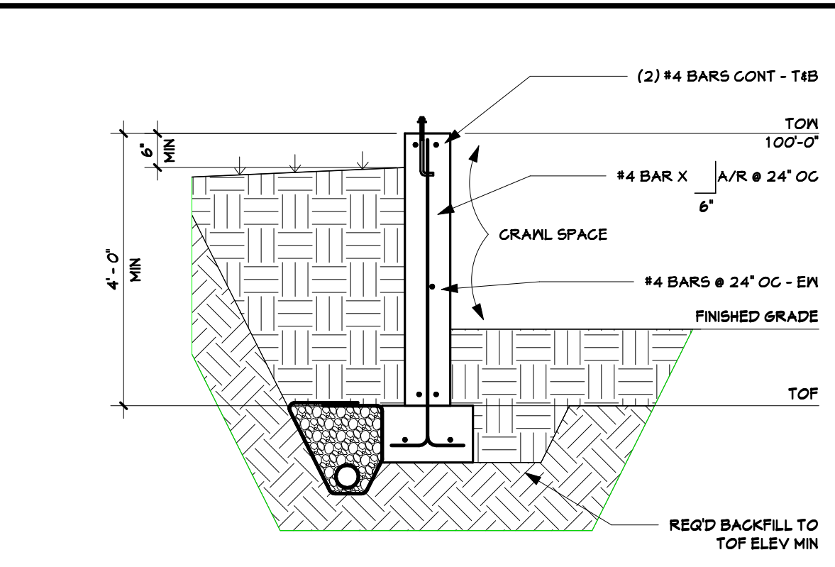
5 CRWL SPACE WALL 1/2" = 1'-0"
