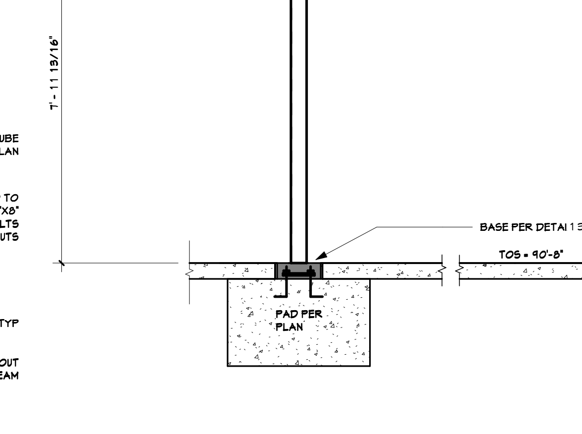
17 BEAM DETAIL 1/2" = 1'-0"
