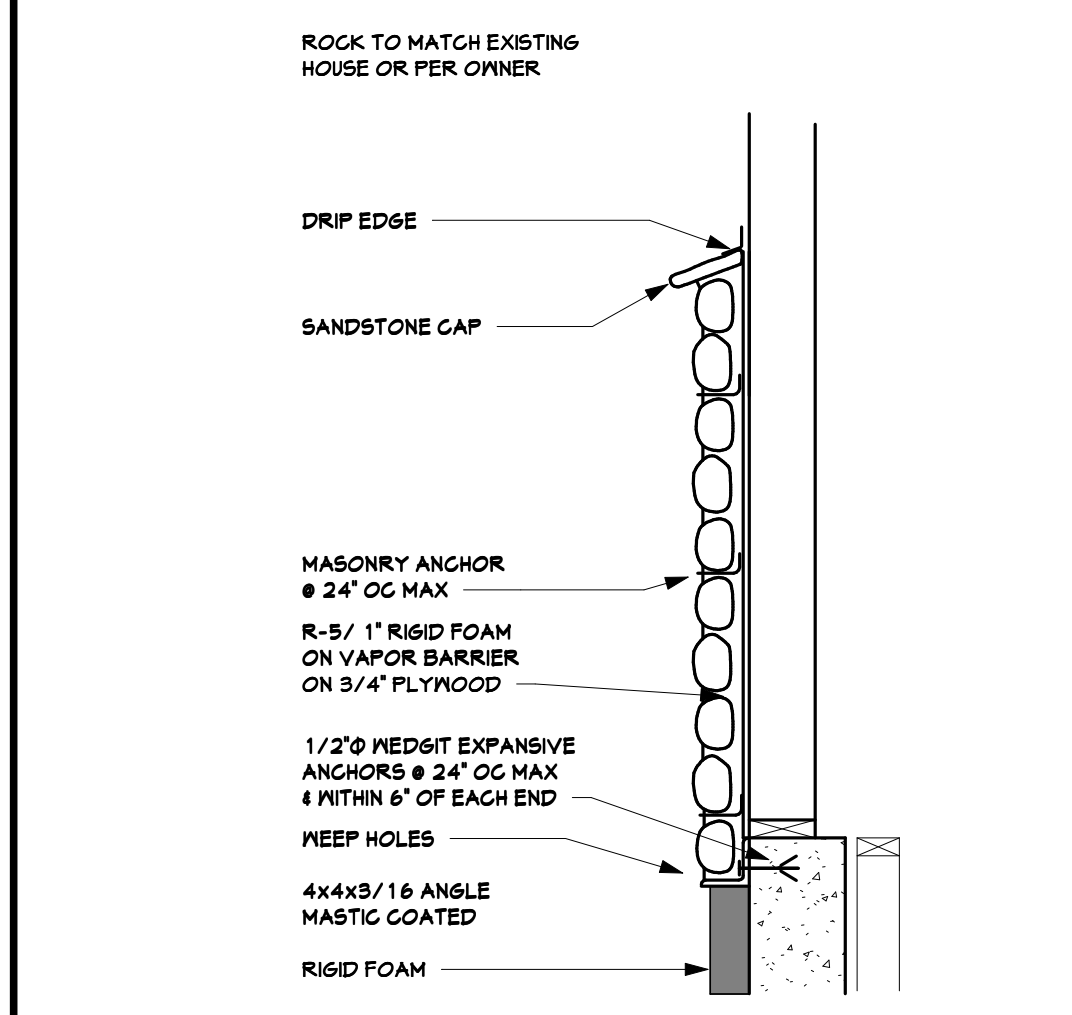
6 RIVER ROCK LEDGE DETAIL 3/4" = 1'-0"
