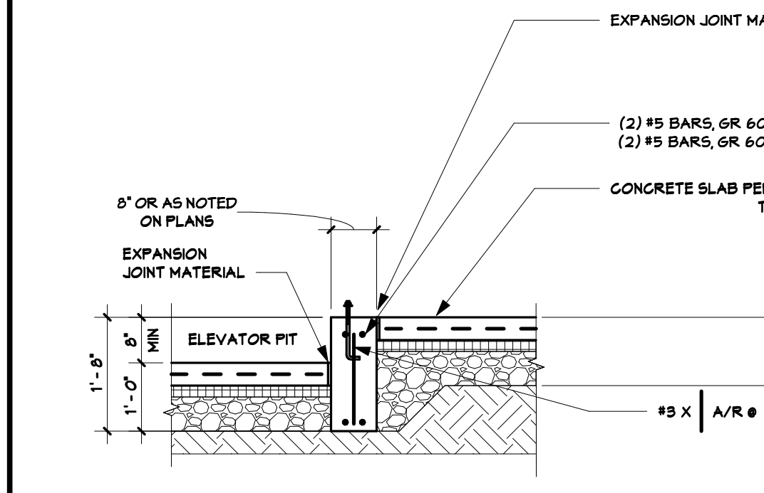
11 CANTILEVERED WALL 1/2" = 1'-0"
