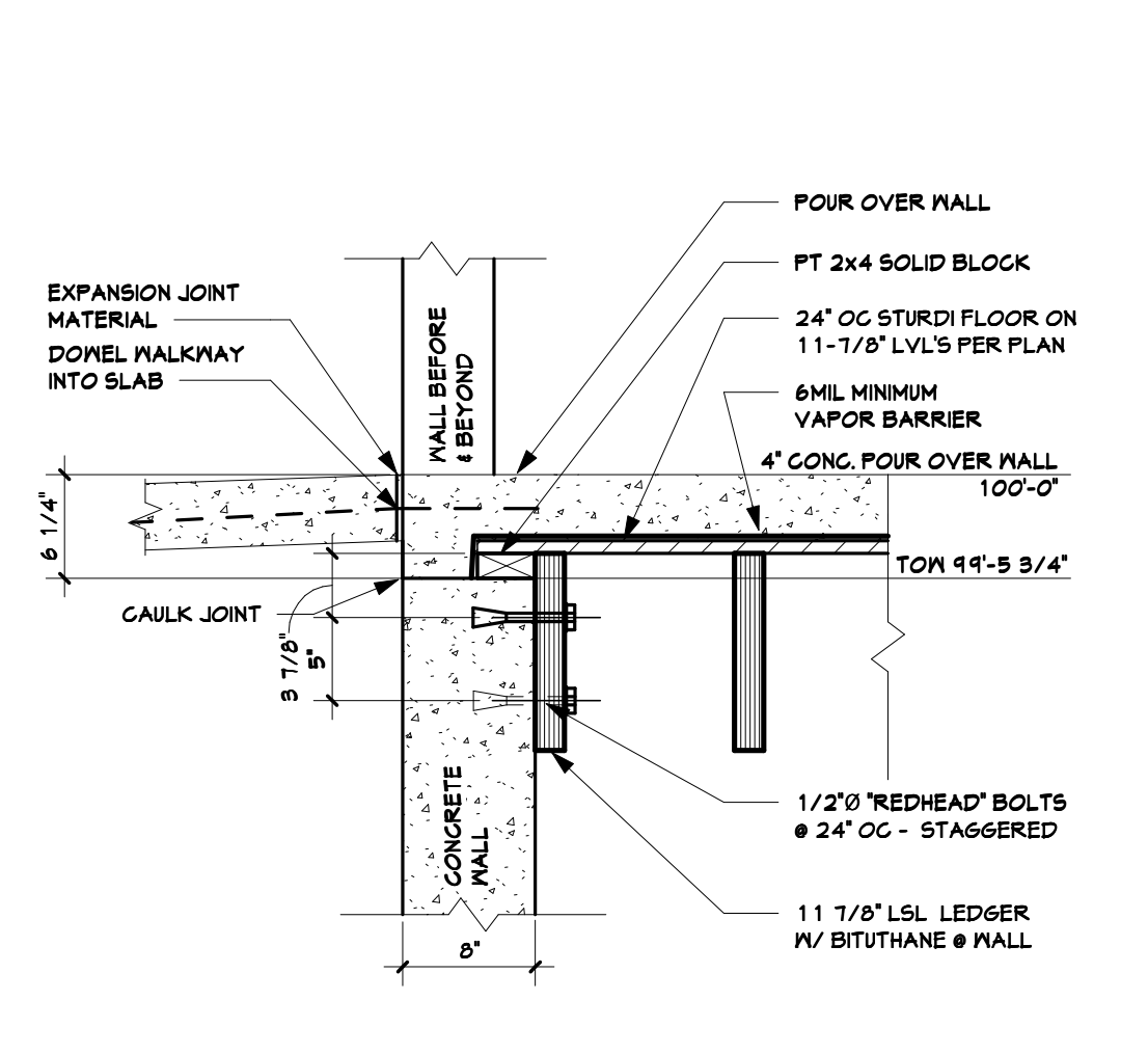
8 NORTH & SOUTH WALL @ DOORS 1" = 1'-0"
