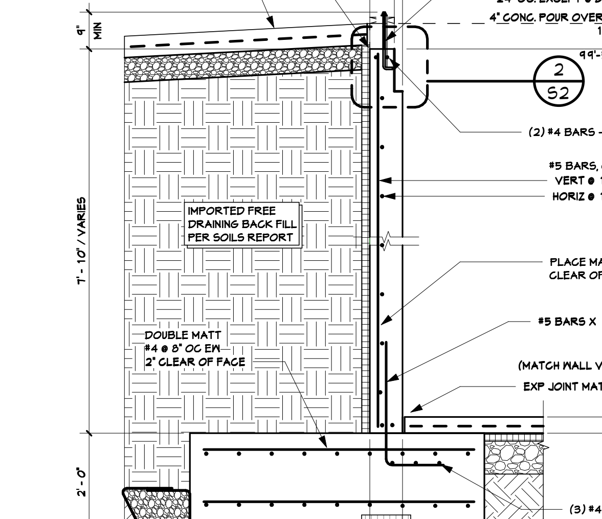
10 UNDERSLAB ISOLATED PAD 1/2" = 1'-0"
