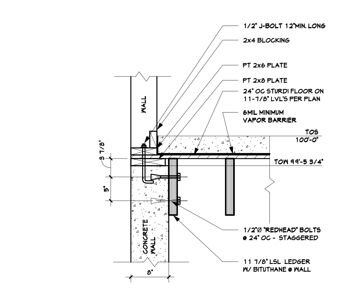
7 NORTH & SOUTH WALL 1" = 1'-0"
