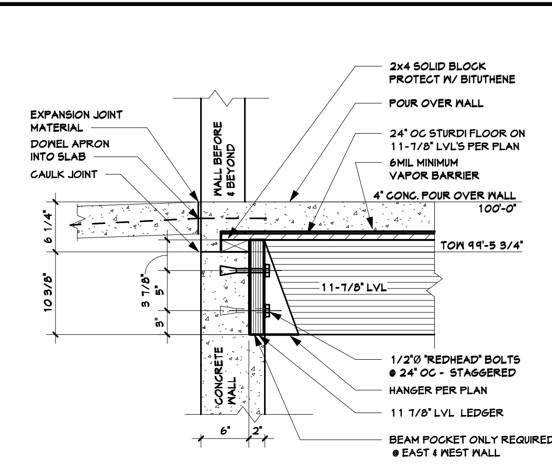
3 WEST & EAST WALL @ DOORS 1" = 1'-0"
