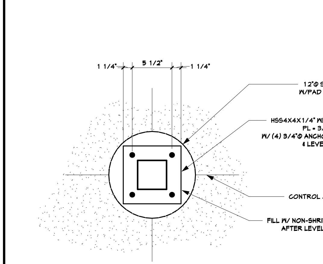
16 STEEL BASE HSS4X4 1 1/2" = 1'-0"
