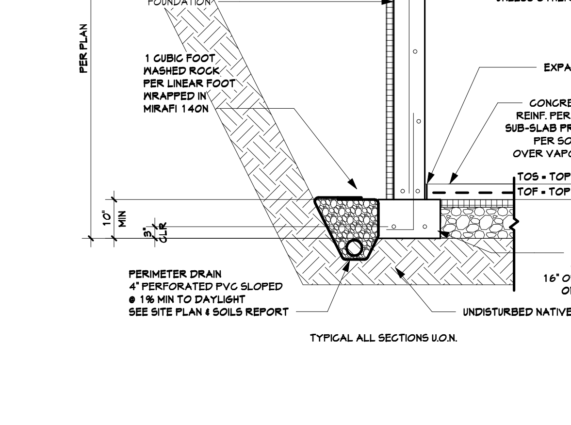
20 WALL, SLAB & FOOTER DETAIL 1/2" = 1'-0"
