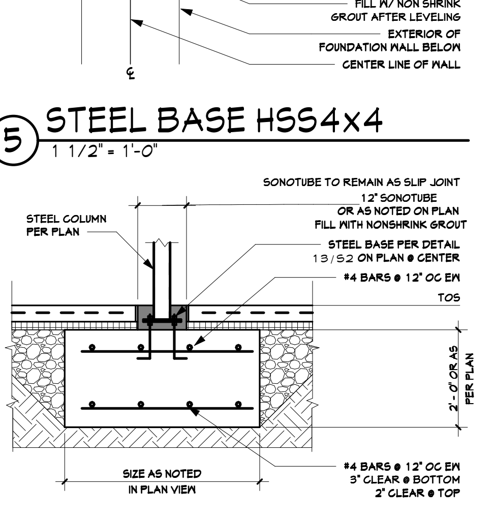
9 STEEL BASE HSS4X4 1 1/2" = 1'-0"
