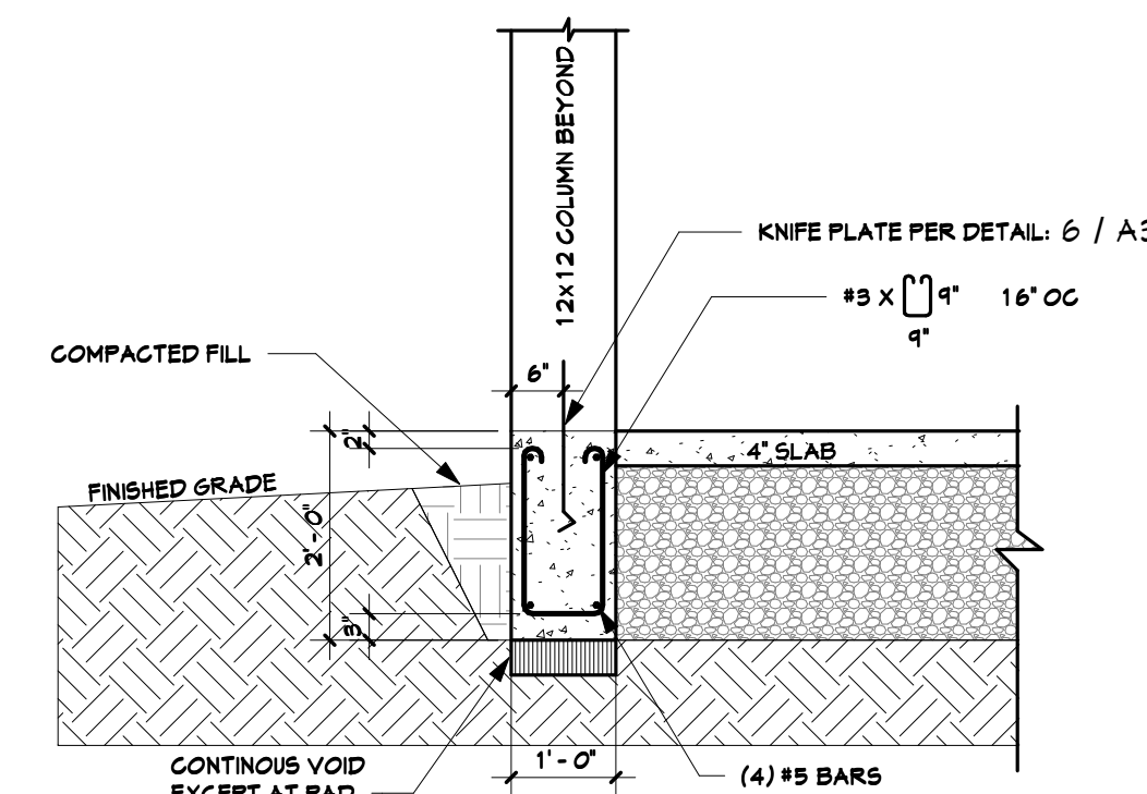
7 12" FOUNDATION WALL 1/2" = 1'-0"
