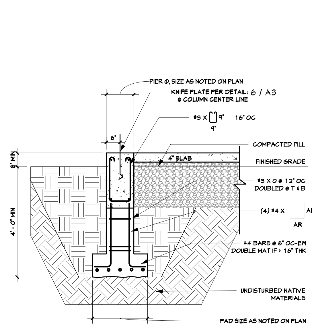
9 EXCAVATED PIER W/ PAD 1/2" = 1'-0"
