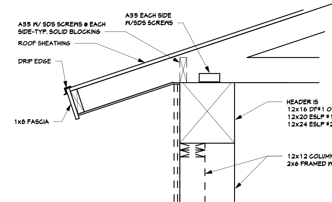
5 SOFFIT VENT DETAIL 1" = 1'-0"
