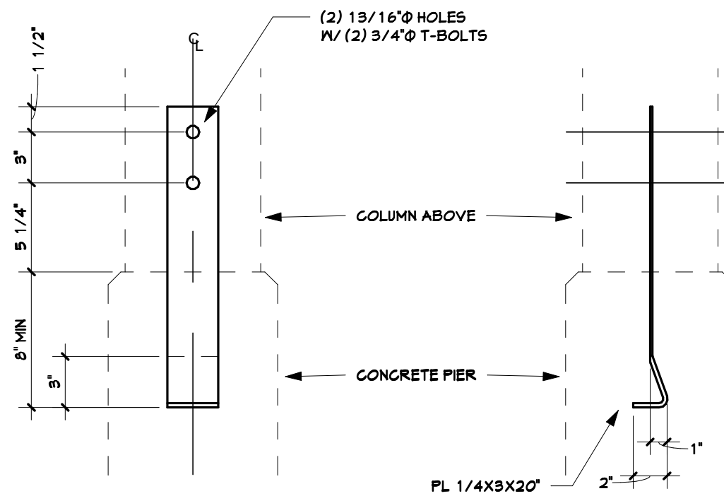
6 KNIFE PLATE 1 1/2" = 1'-0"
