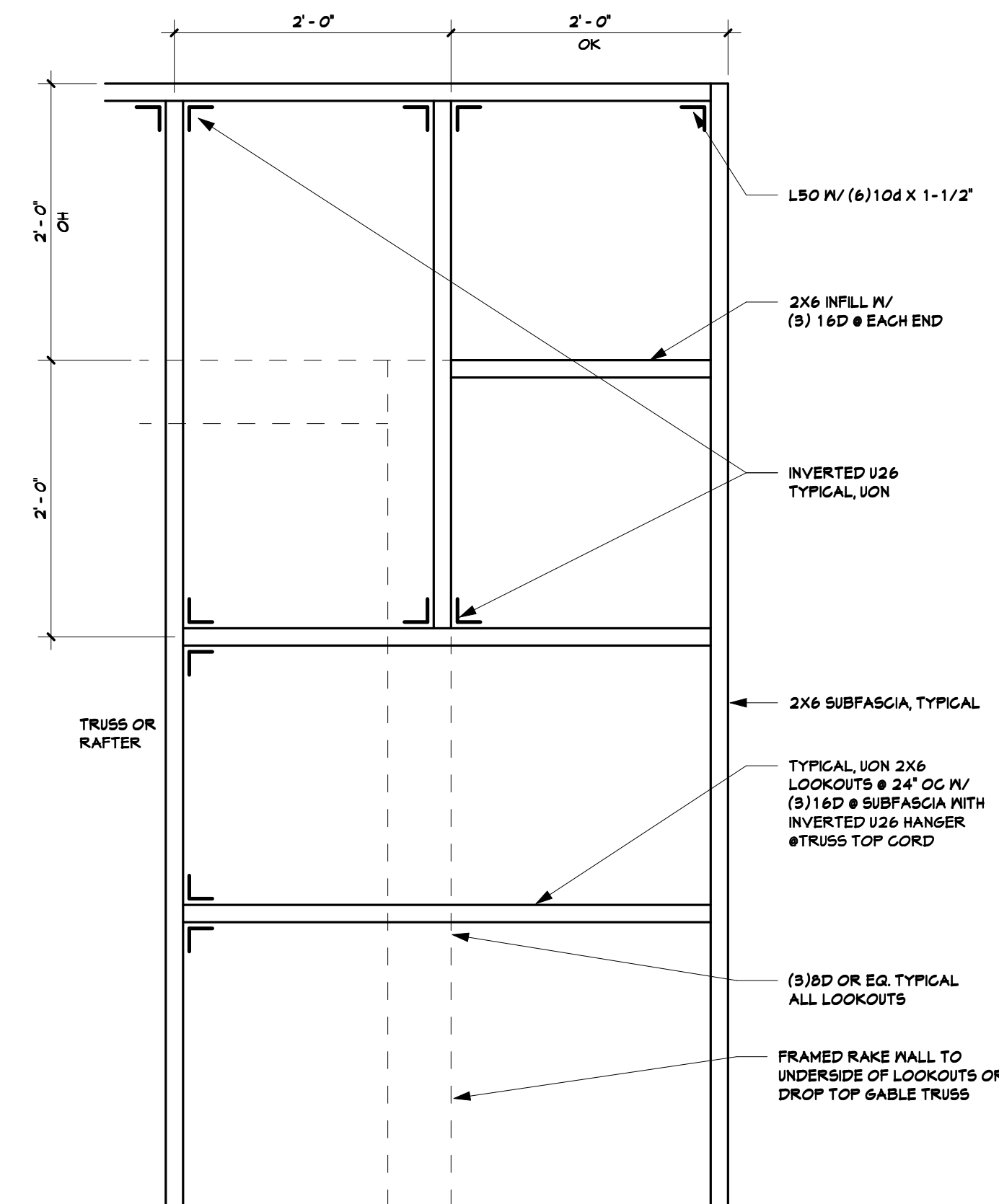
1 CORNER DETAIL 1" = 1'-0"
