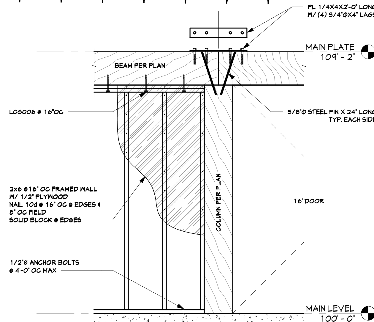
4 BEAM SPLICE WITH SHEAR WALL DETAIL 1/2" = 1'-0"
