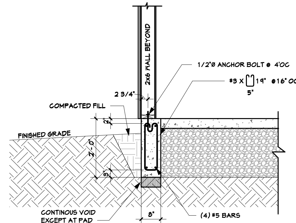
8 8" FOUNDATION WALL 1/2" = 1'-0"
