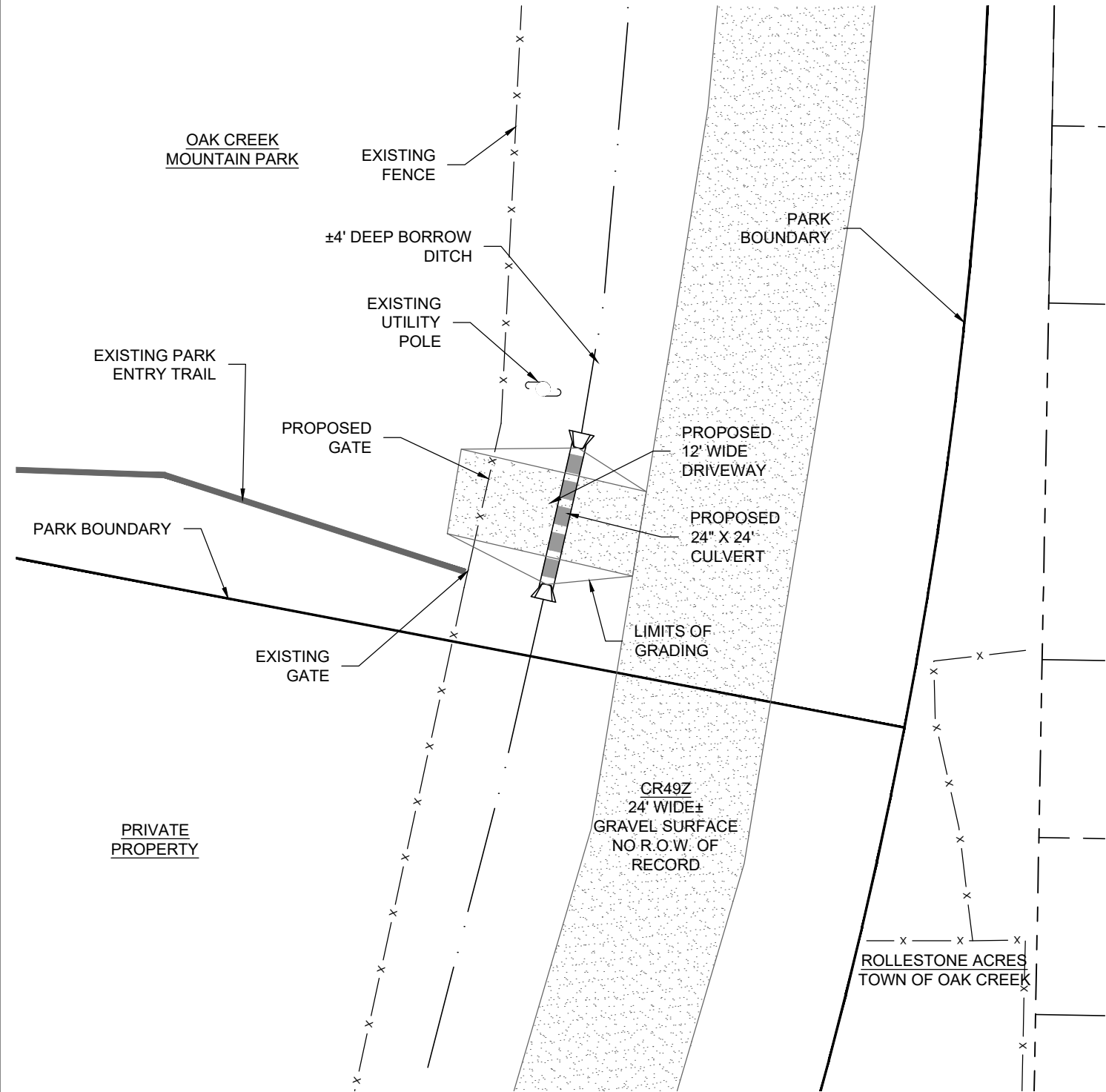
DRIVEWAY PLAN
