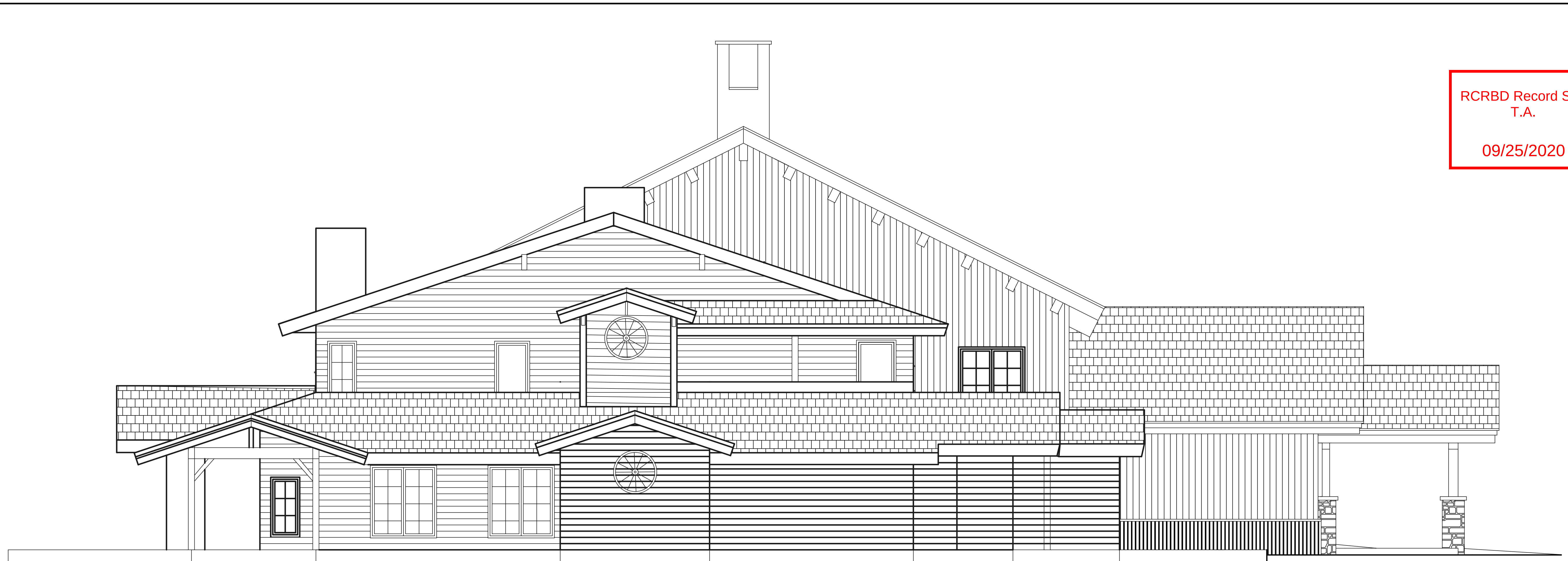
1 A-1 EXISTING NORTH ELEVATION SCALE 1/4" = 1'-0"
