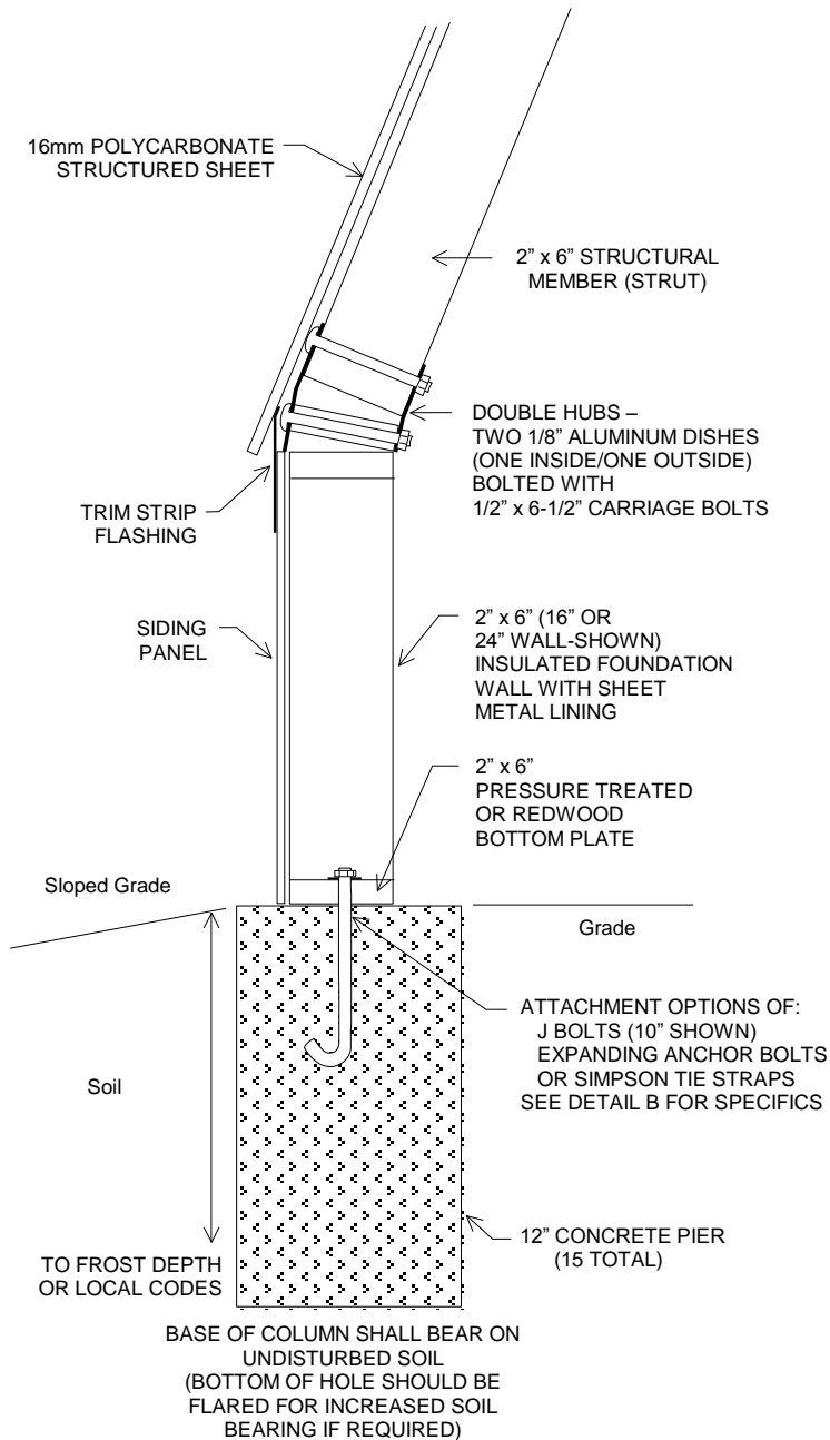
FOUNDATION DETAIL AT PIER
