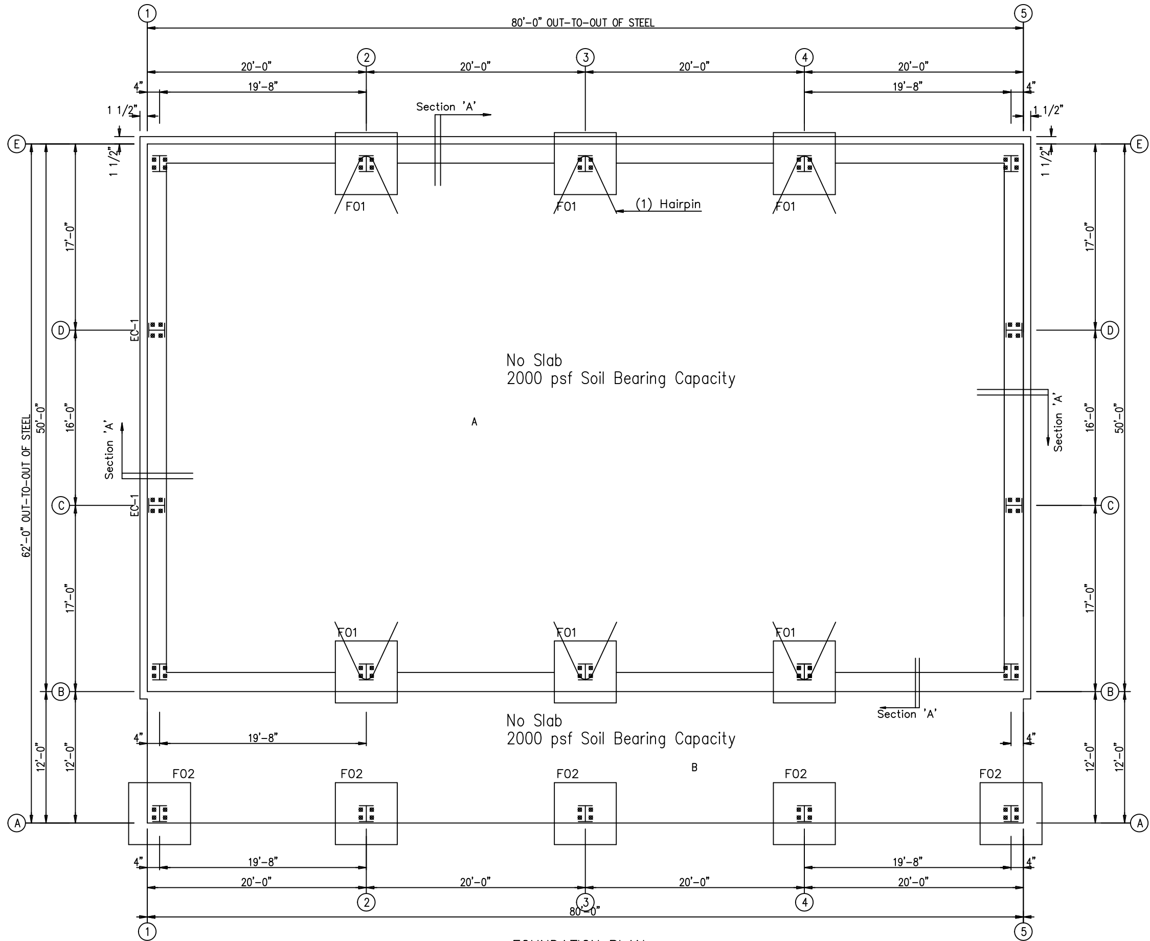
FOUNDATION PLAN NOTE: Not to Scale
