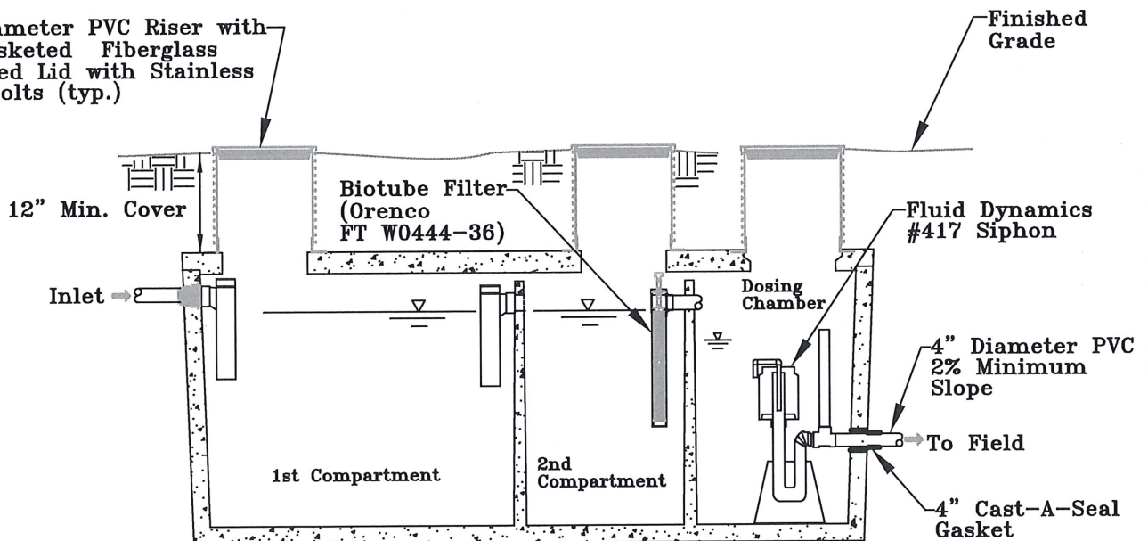
Section View
