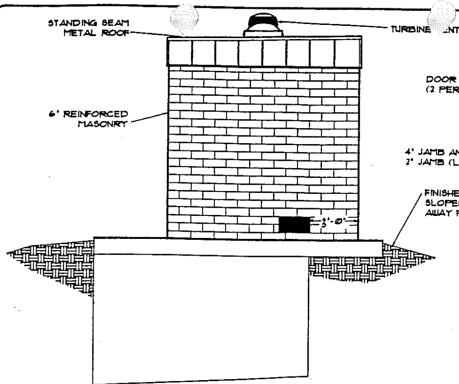
A 3 LEFT SIDE ELEVATION SCALE: 1/4" = 1 FOOT
