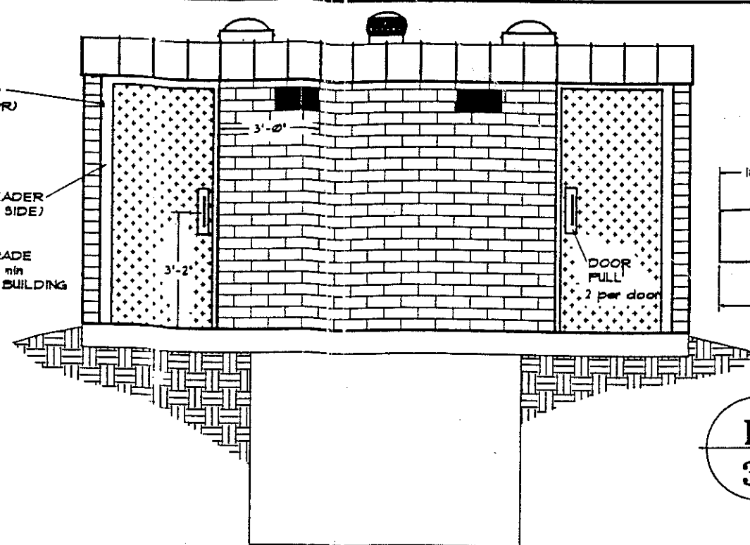
C 3 FRONT ELEVATION SCALE: 1/4" = 1 FOOT
