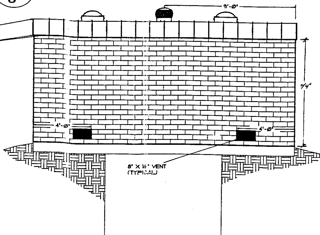
D 3 REAR ELEVATION SCALE: 1/4" = 1 FOOT
