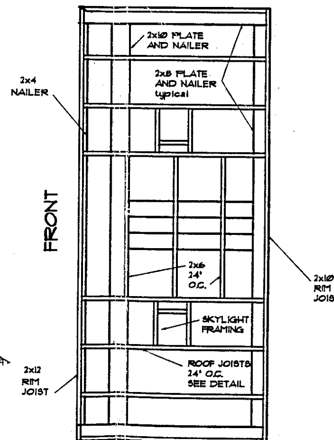
E 3 ROOF JOIST NO SCALE
