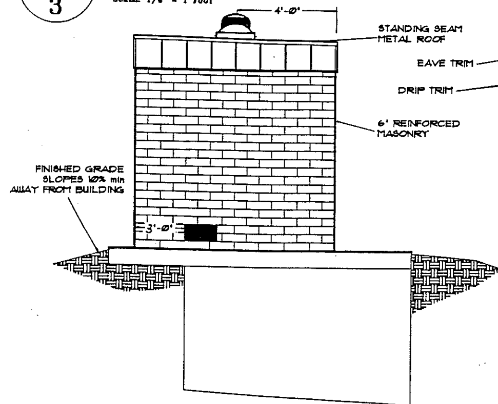
B 3 RIGHT SIDE ELEVATION SCALE: 1/4" = 1 FOOT
