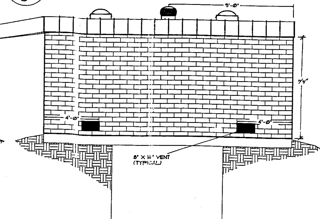
D 3 REAR ELEVATION SCALE: 1/4" = 1 FOOT
