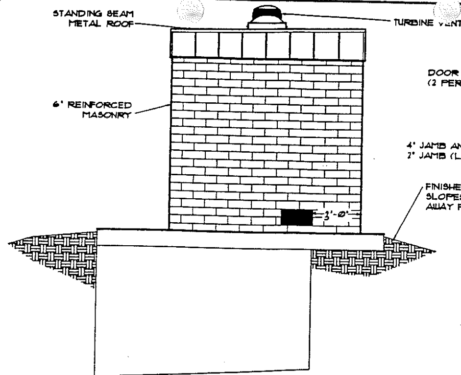
A 3 LEFT SIDE ELEVATION SCALE: 1/4" = 1 FOOT
