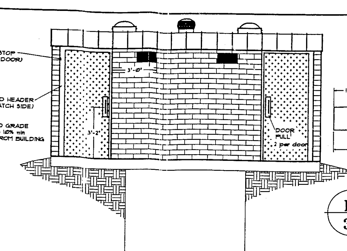
C 3 FRONT ELEVATION SCALE: 1/4" = 1 FOOT
