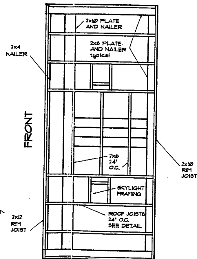
E 3 ROOF JOIST NO SCALE
