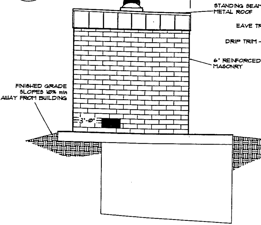
B 3 RIGHT SIDE ELEVATION SCALE: 1/4" = 1 FOOT
