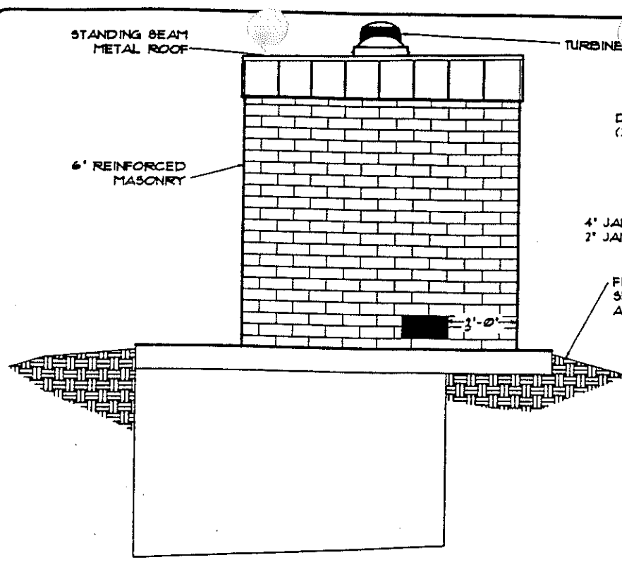
A 3 LEFT SIDE ELEVATION SCALE: 1/4" = 1 FOOT
